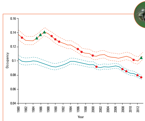
Patterns of change in the ranges of wild bees (blue) and hoverflies (orange). Trend lines show average occupancy of 1 km grid cells in Britain across all modelled bee ( n = 139 ) and hoverfly ( n = 214 ) species. Red circles and green triangles highlight years with notable decreases or increases, respectively [Powney et al. 2019].
